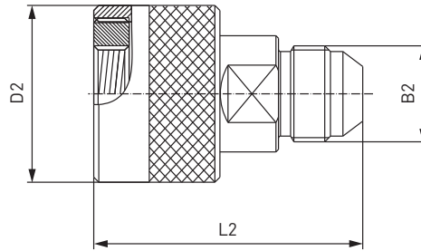
Connector with media inlet (SAE J512, J513, J514)
