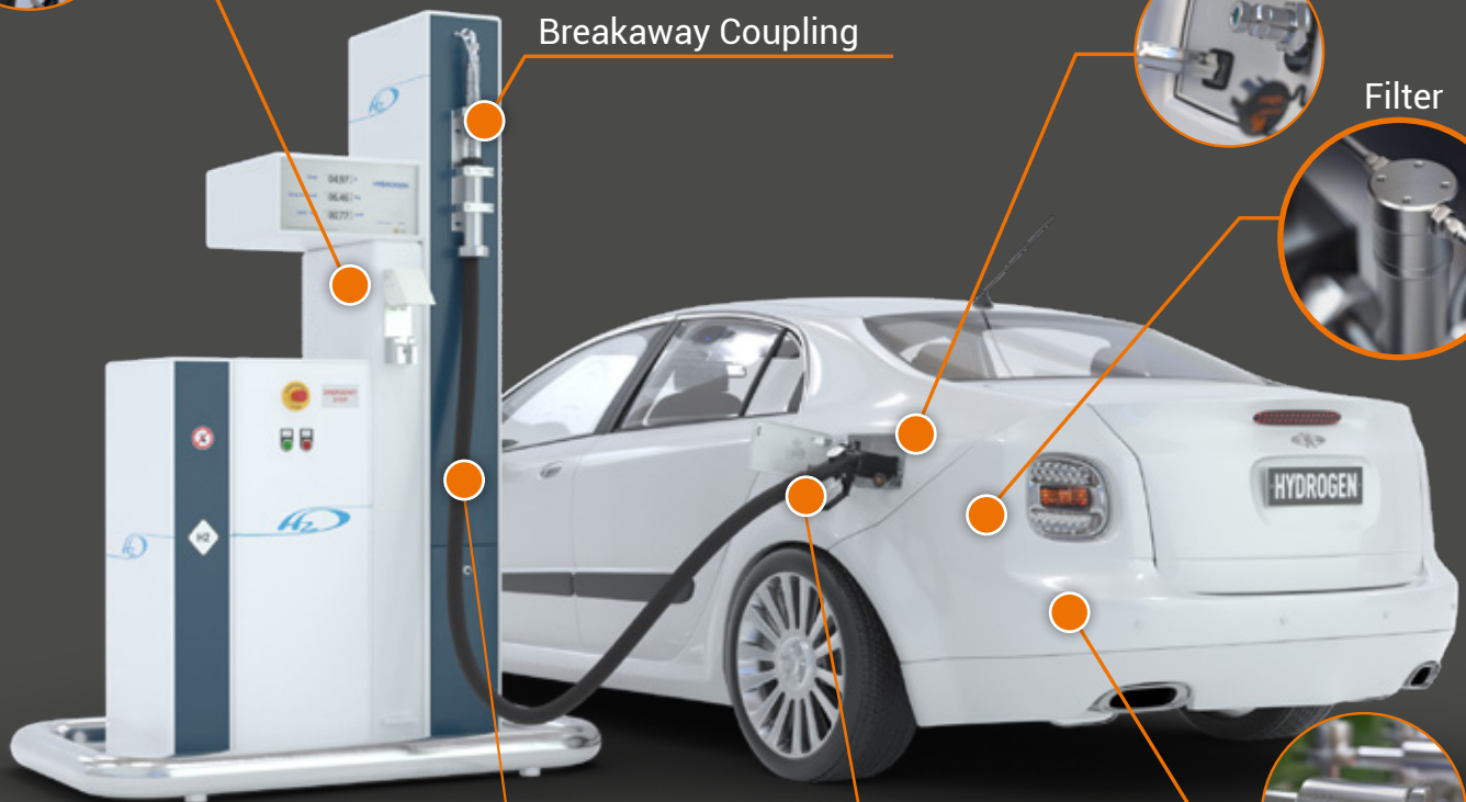
Hose Assembly
